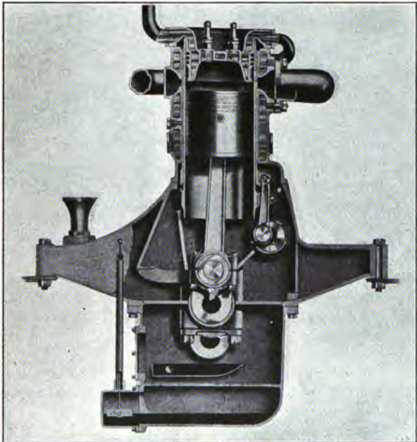
FIG. 70b. —Columbia Knight Motor, Cross-Section View.
